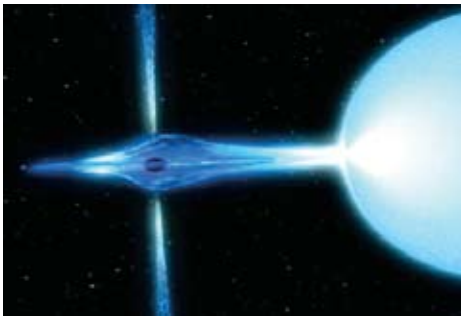
Material from a normal companion star falls onto a black hole forming an accretion disk and outflowing jets of material - NASA/Honeywell Max-Q Digital Group.
